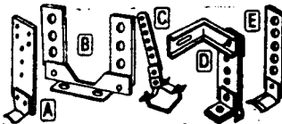
MUFFLER CLIPS (387)
