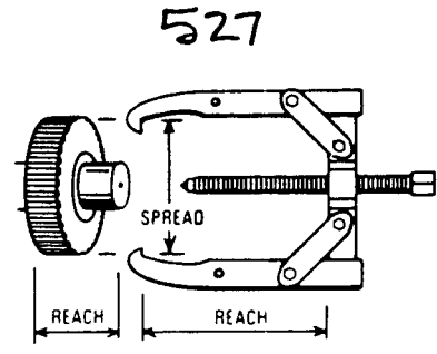
PLATE PULLER
