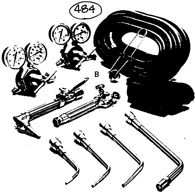
OXY-ACETYLENE WELDER
