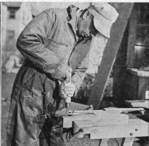
Vise on corner of jointercart worktable is handy accessory. Since jointer isn't flush with side of frame, vise can handle long work.
